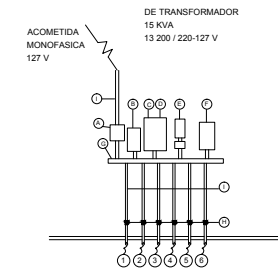
DETALLE No. 1 CONTROL ELECTRICO (S/E)
